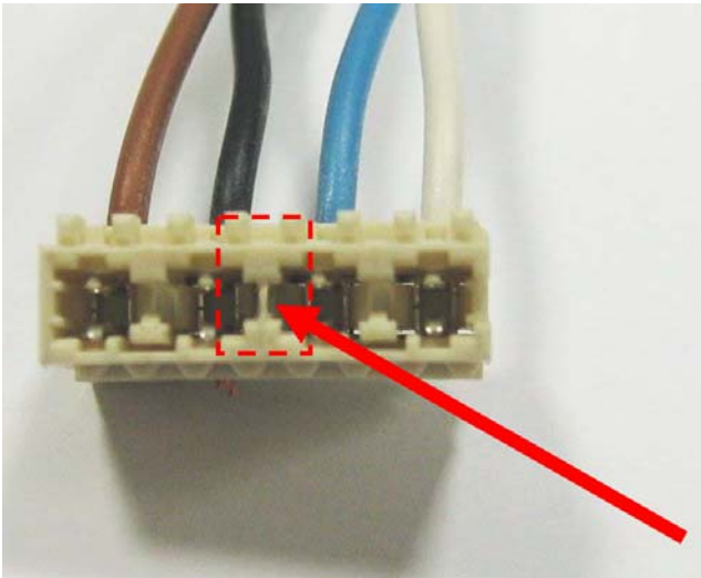
a) Identify the plastic tab positioned inside the 4-pole connector J2 as indicated by the arrow in figure.
