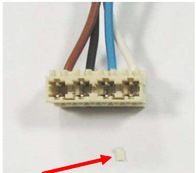
d) Remove the plastic tab from the connector.
